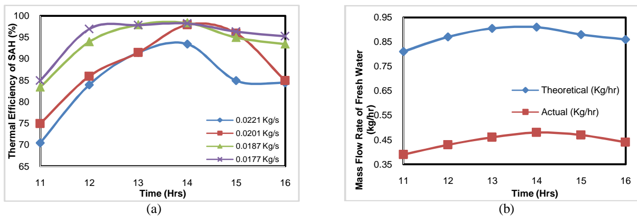
Fig. 4. (a) Thermal Efficiency of SAH for Different Mass Flow Rate (b) Comparison Actual rate of water outcome with Theoretical
