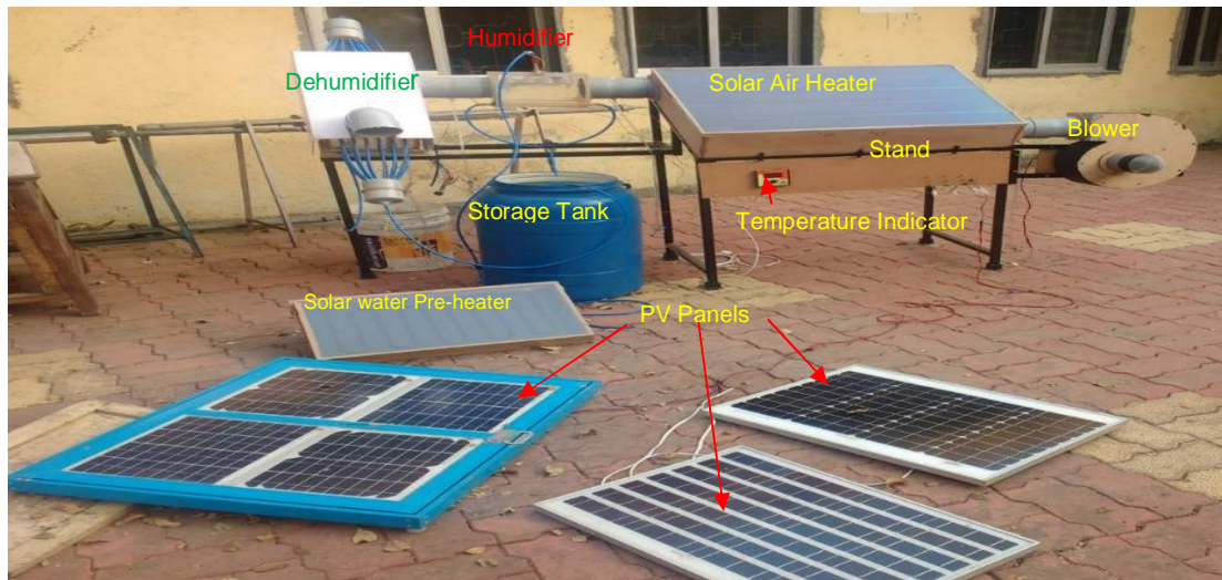
Fig. 2. Photograph of Experimental Set-Up
