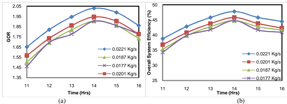
Fig. 5. (a) GOR for Different Mass Flow Rate (b) Overall System Efficiency at Different Mass Flow Rate
